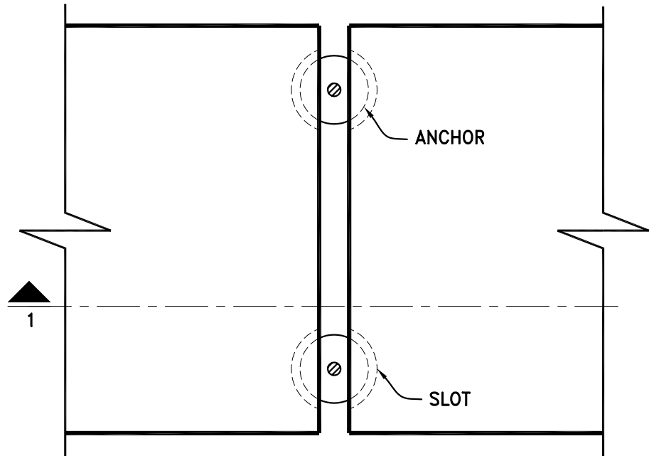
3 HORIZONTAL SECTION
